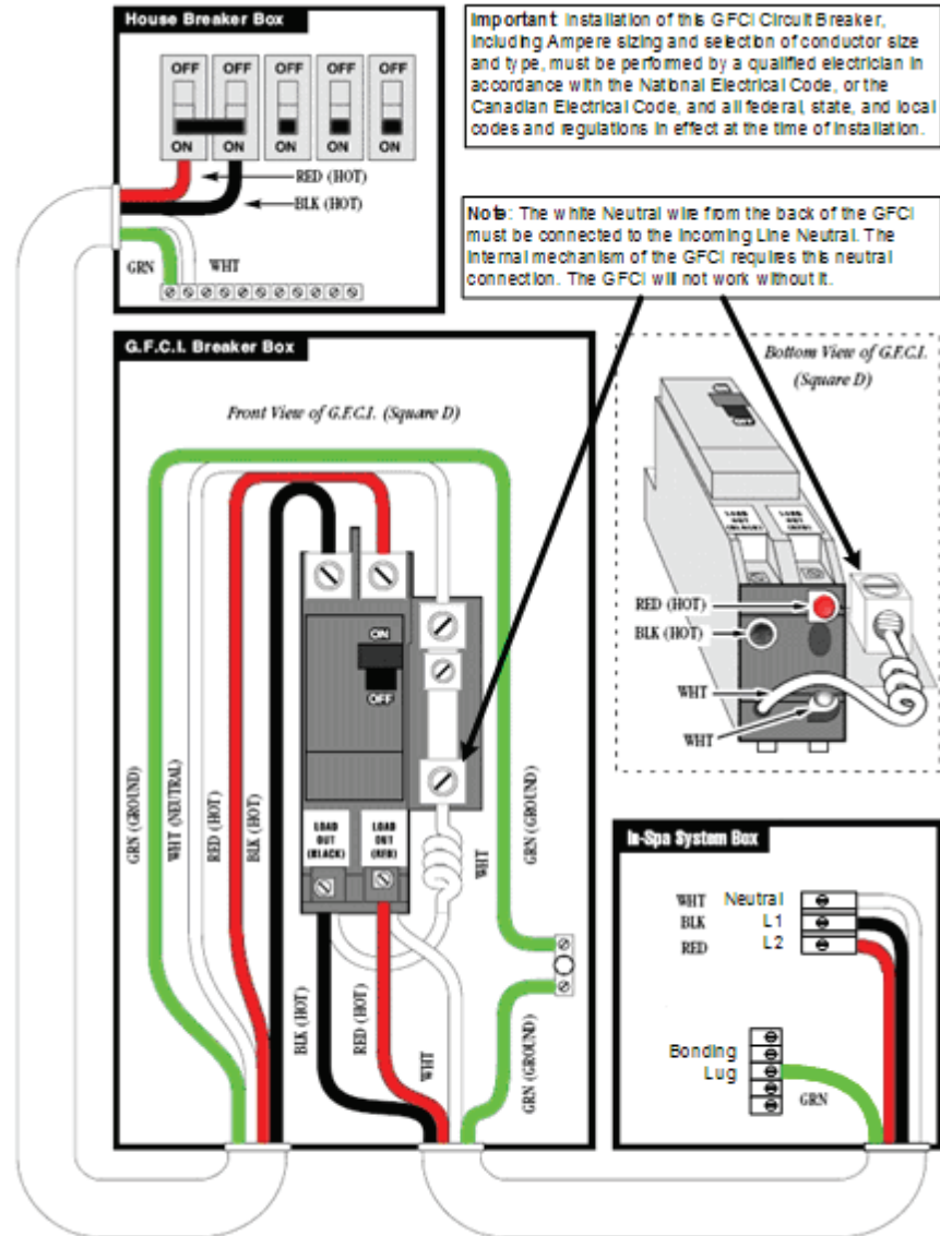
Figure 4 – Electrical Service for all domestic Single-phase 240vac models
